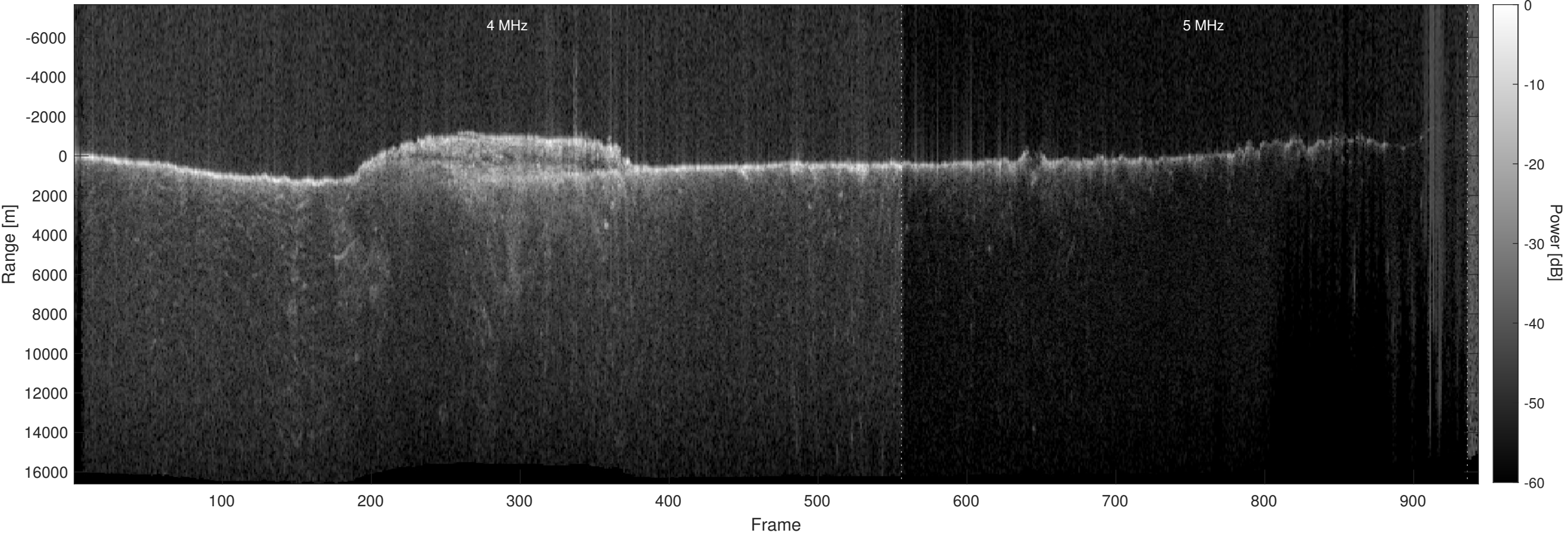
Orbit 11737, Optimized, Window, Depth-Corrected, Channel 2
