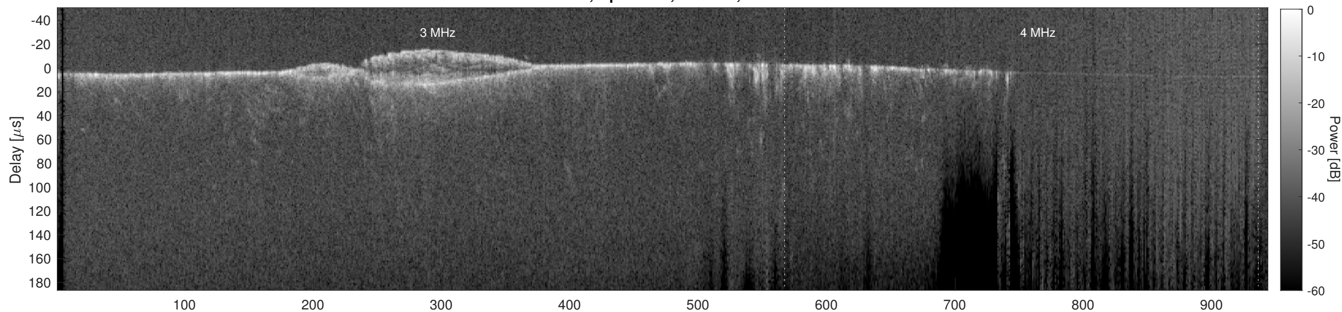
Orbit 11740, Cluttergram
