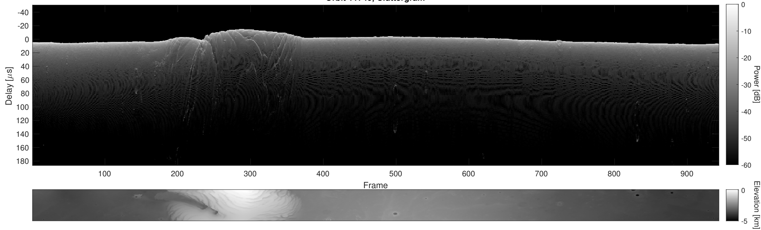
Orbit 11740, Cluttergram
