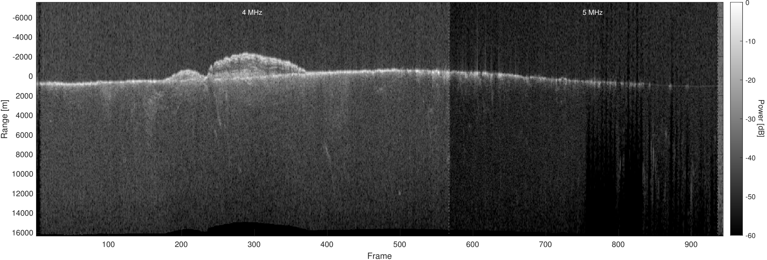
Orbit 11740, Optimized, Window, Depth-Corrected, Channel 2
