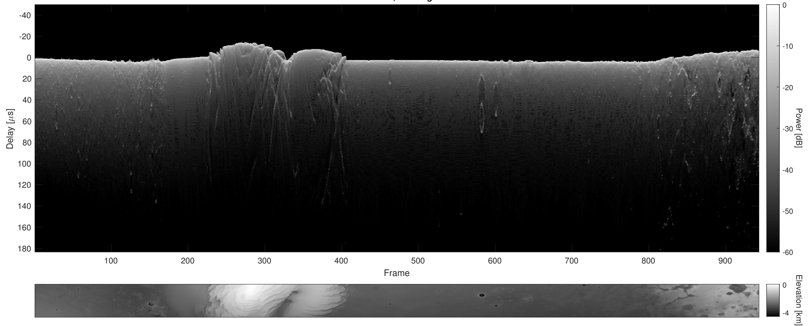
Orbit 11741, Cluttergram
