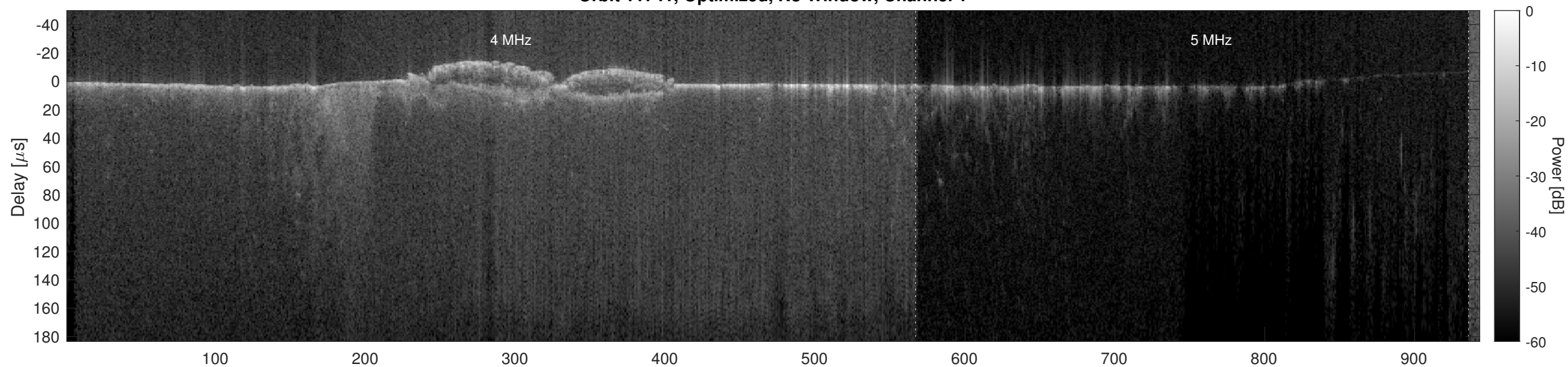
Orbit 11741, Optimized, No Window, Channel 2
