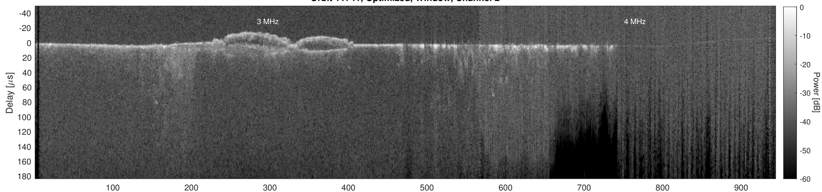
Orbit 11741, Cluttergram
