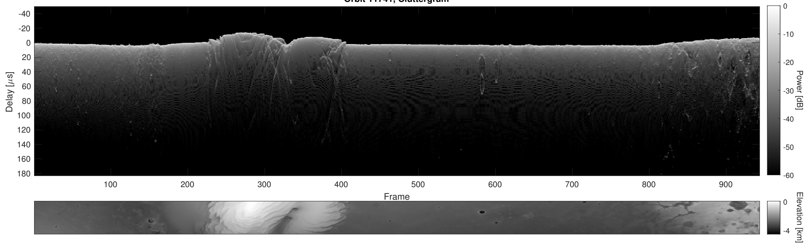
Orbit 11741, Cluttergram
