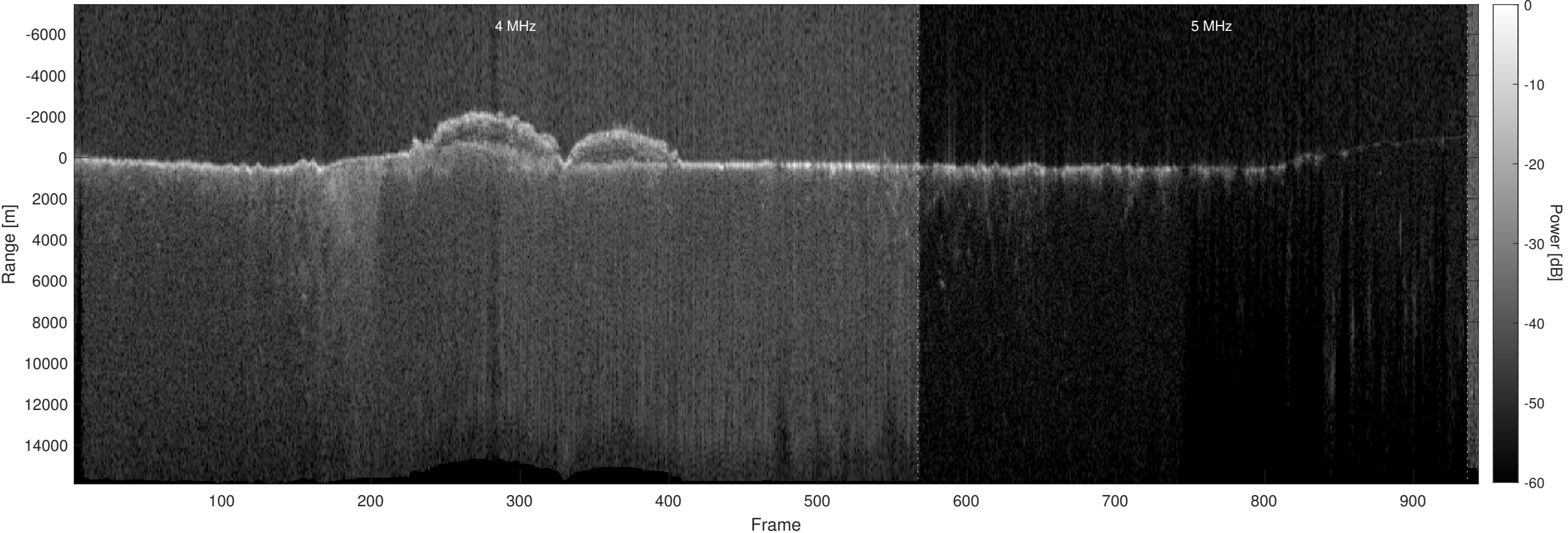
Orbit 11741, Optimized, Window, Depth-Corrected, Channel 2
