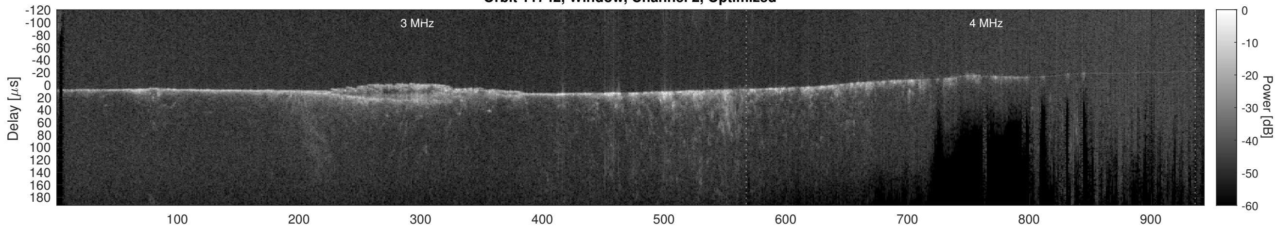
Orbit 11742, Cluttergram
