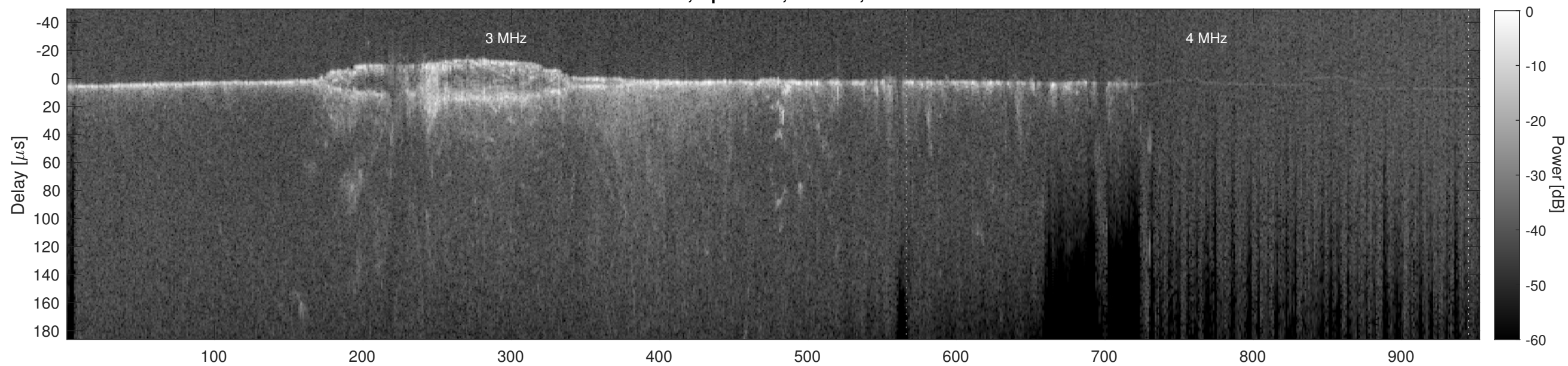
Orbit 11743, Cluttergram
