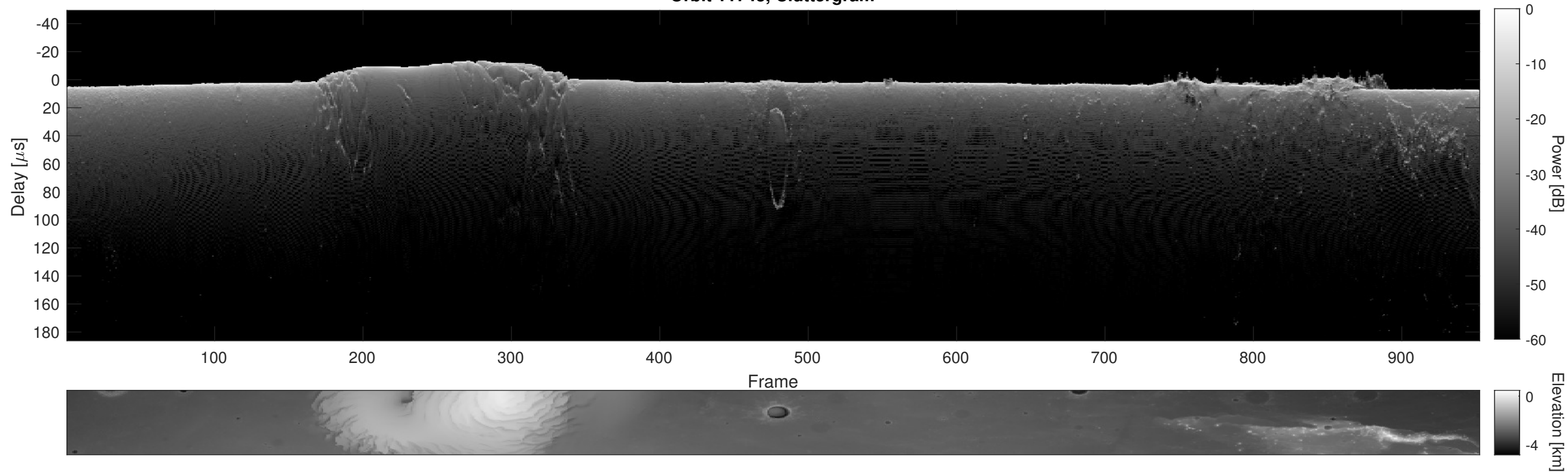
Orbit 11743, Cluttergram
