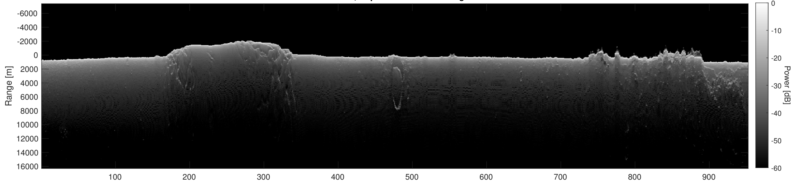
Orbit 11743, Depth-Corrected Cluttergram
