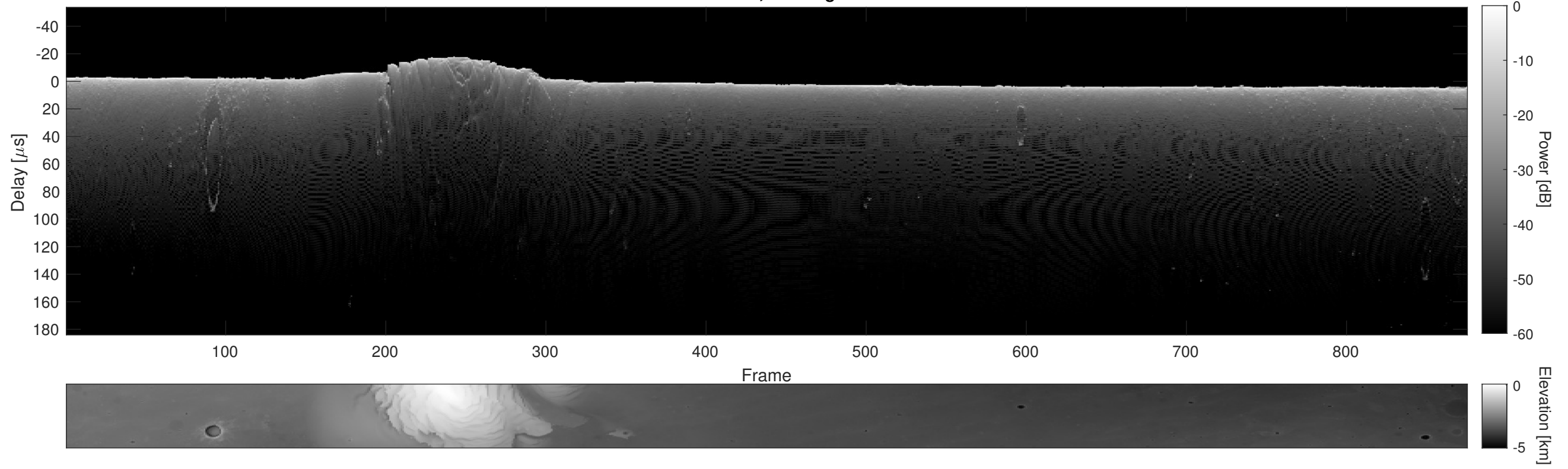
Orbit 11745, Cluttergram
