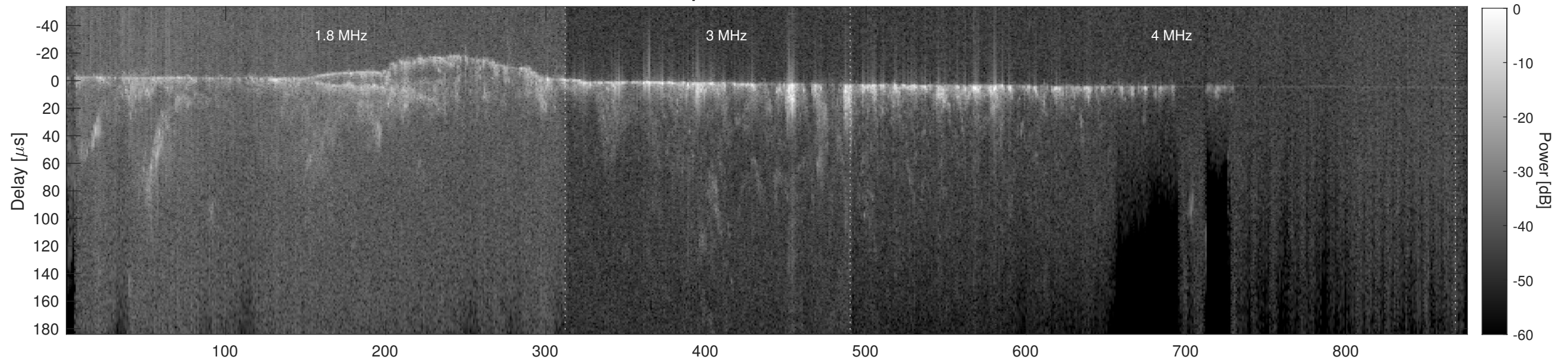
Orbit 11745, Cluttergram
