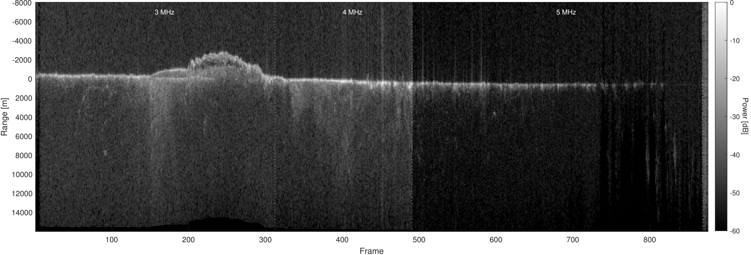
Orbit 11745, Optimized, Window, Depth-Corrected, Channel 2
