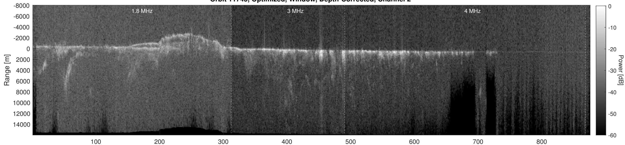
Orbit 11745, Depth-Corrected Cluttergram
