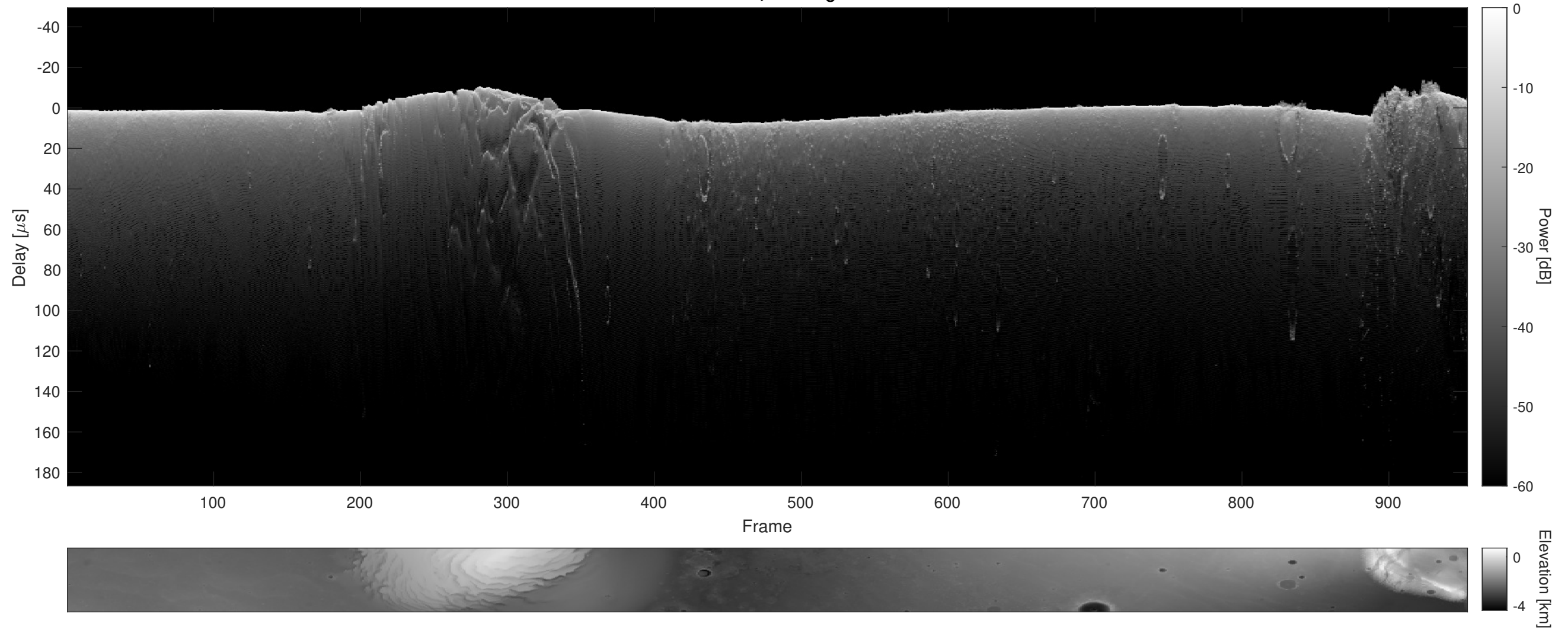
Orbit 11746, Cluttergram
