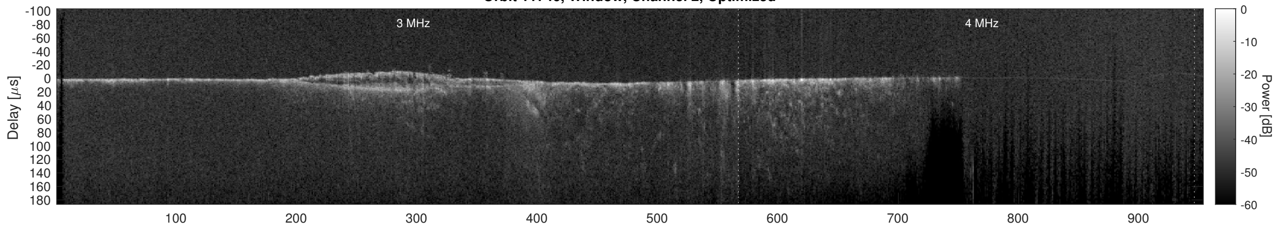
Orbit 11746, Cluttergram
