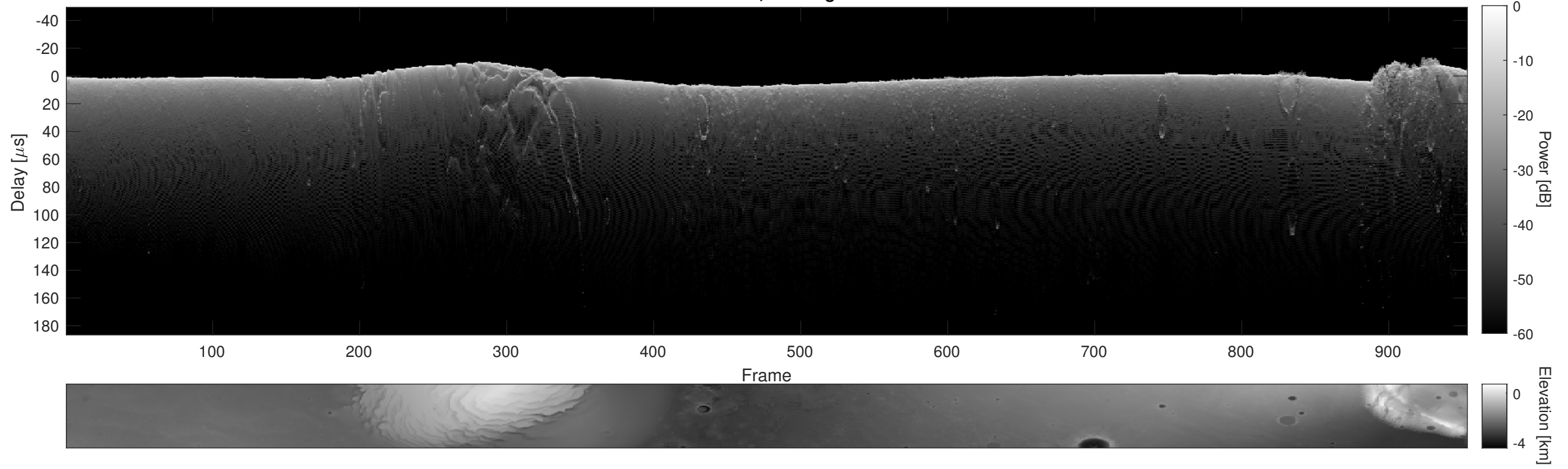
Orbit 11746, Cluttergram
