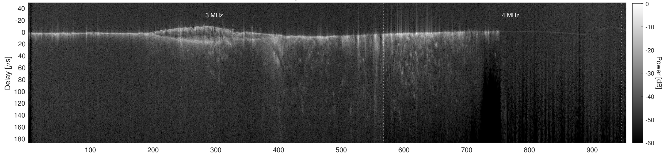
Orbit 11746, Cluttergram
