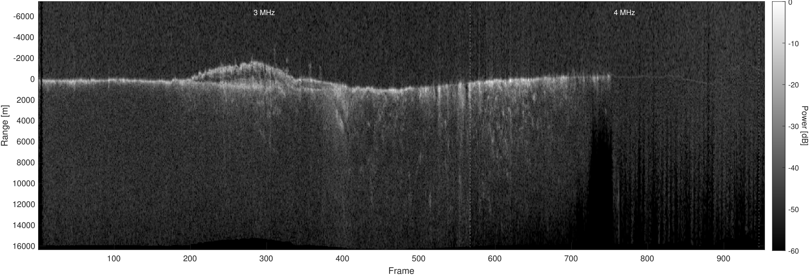
Orbit 11746, Optimized, Window, Depth-Corrected, Channel 2
