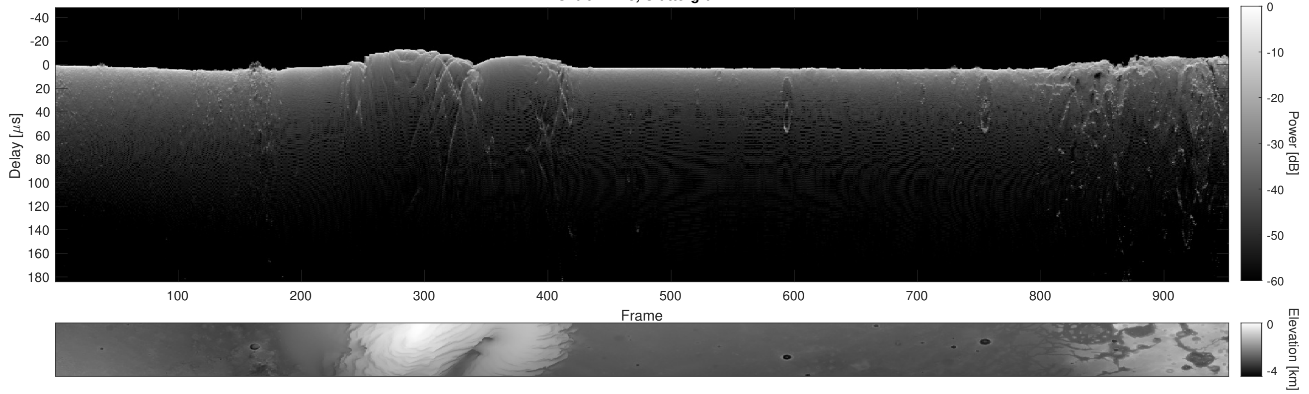
Orbit 11748, Cluttergram
