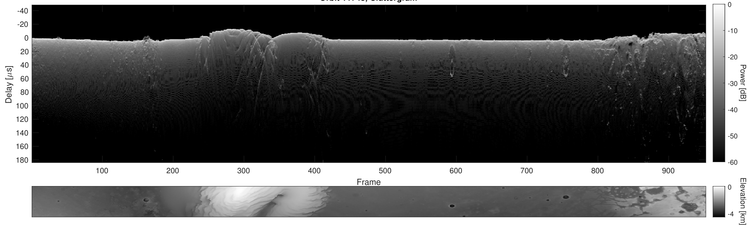
Orbit 11748, Cluttergram
