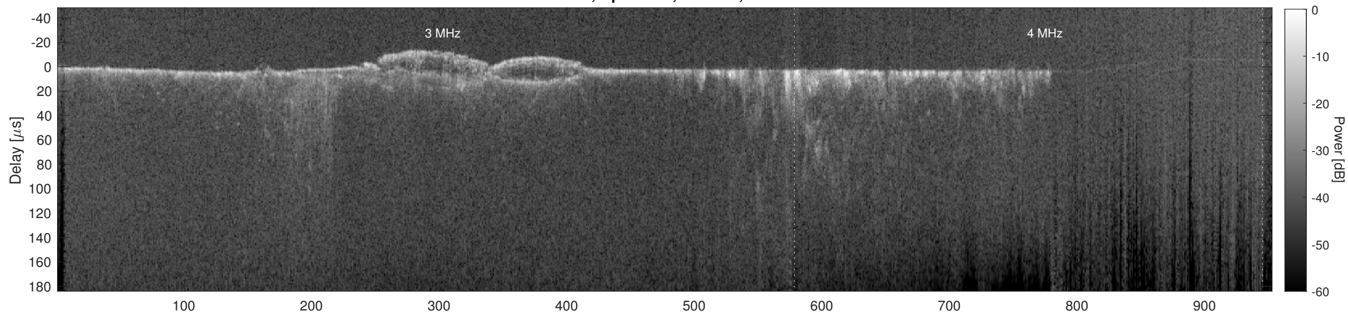
Orbit 11748, Cluttergram
