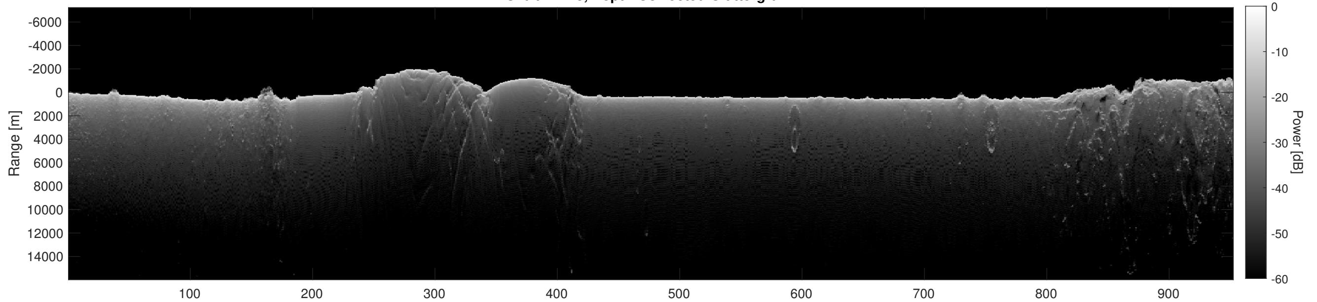
Orbit 11748, Depth-Corrected Cluttergram
