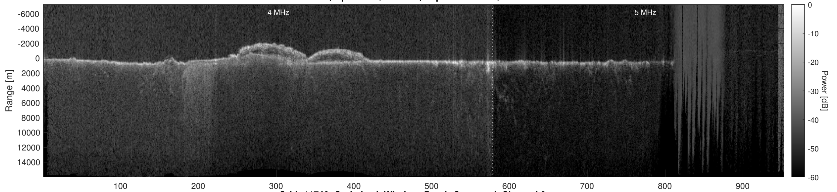
Orbit 11748, Optimized, Window, Depth-Corrected, Channel 2
