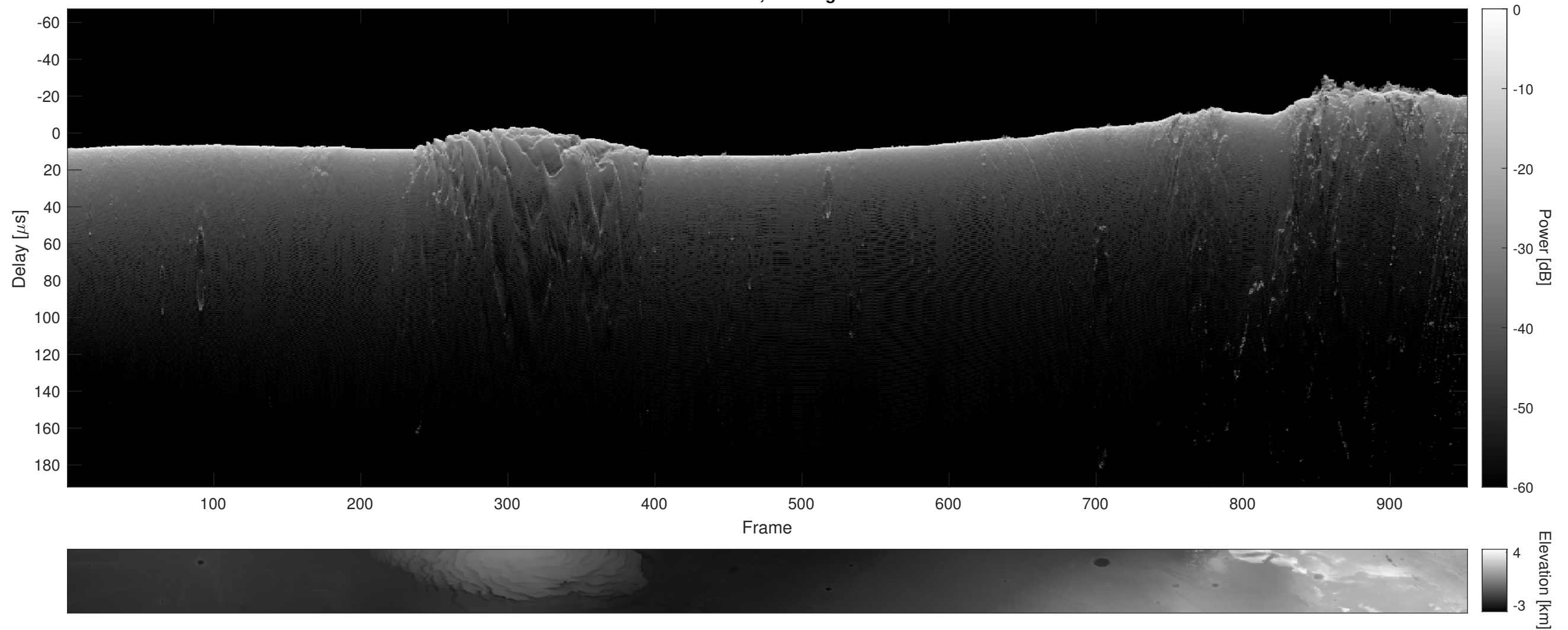
Orbit 11749, Cluttergram
