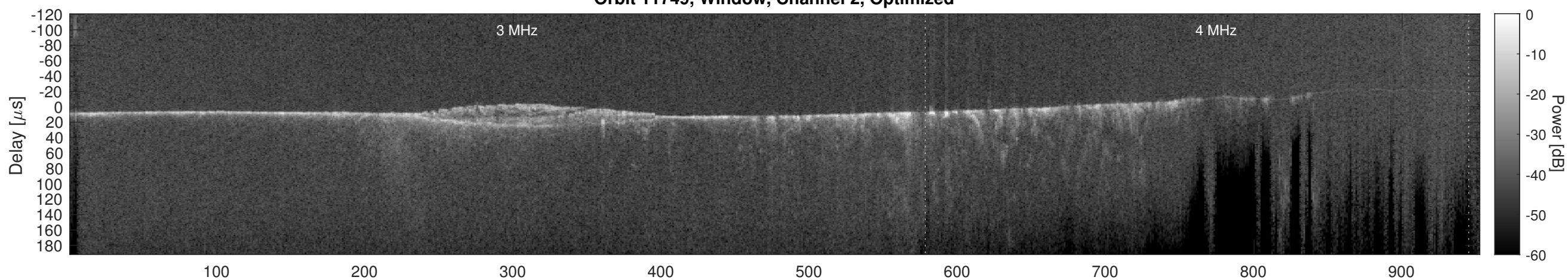
Orbit 11749, Cluttergram
