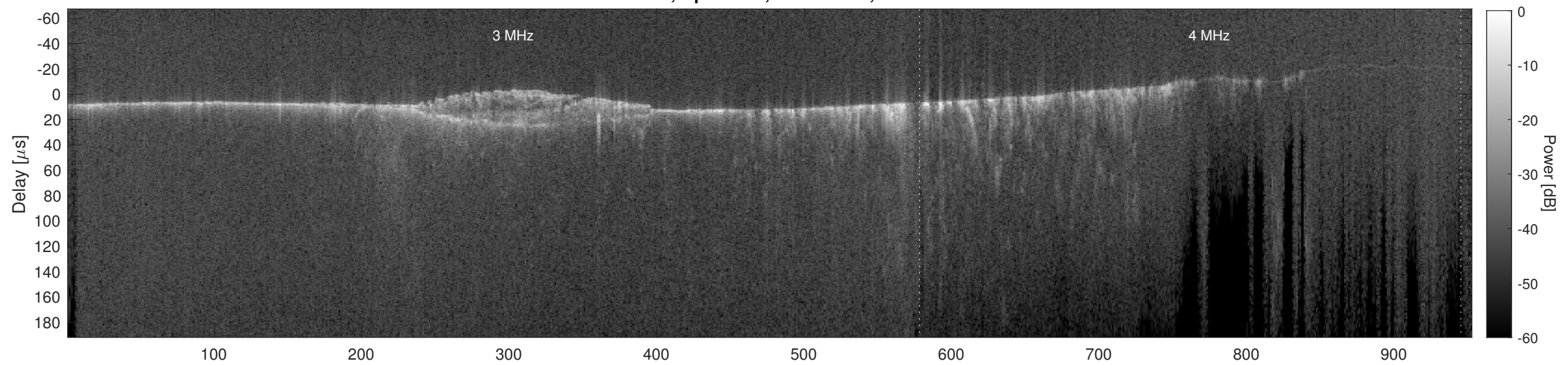
Orbit 11749, Cluttergram
