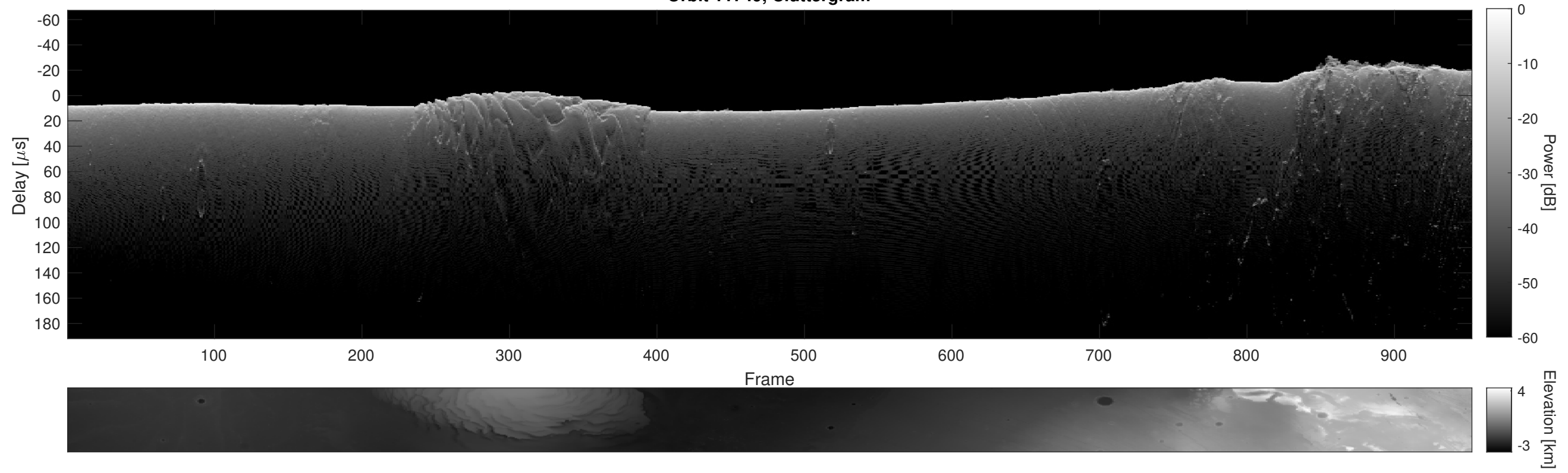
Orbit 11749, Cluttergram
