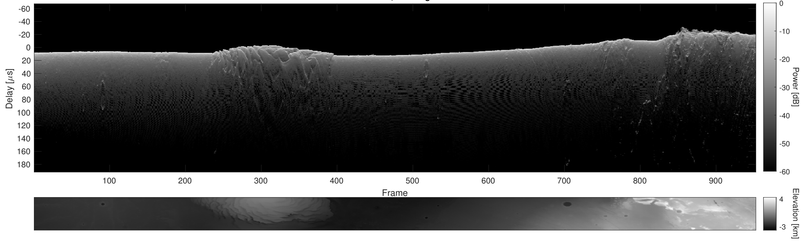
Orbit 11749, Cluttergram
