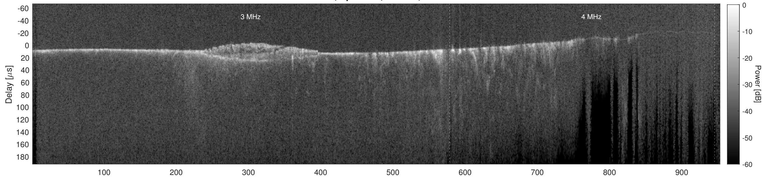
Orbit 11749, Cluttergram
