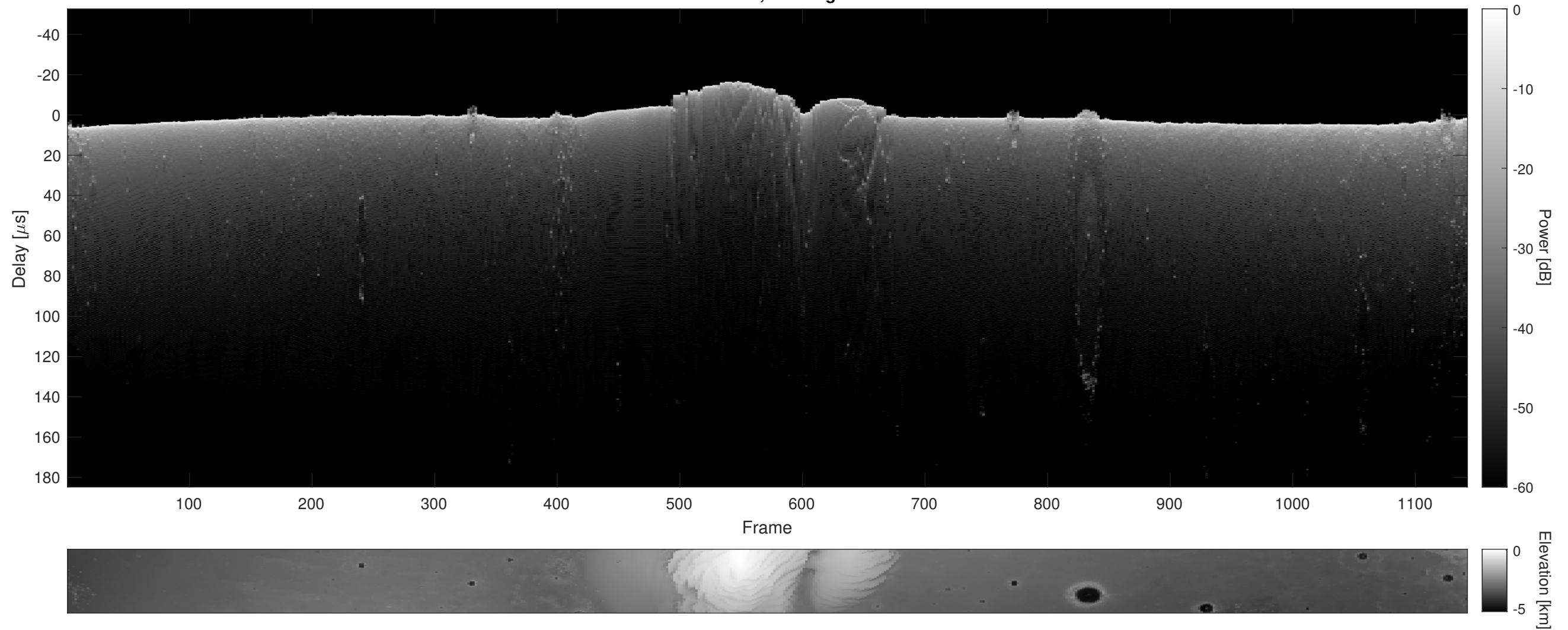
Orbit 11875, Cluttergram
