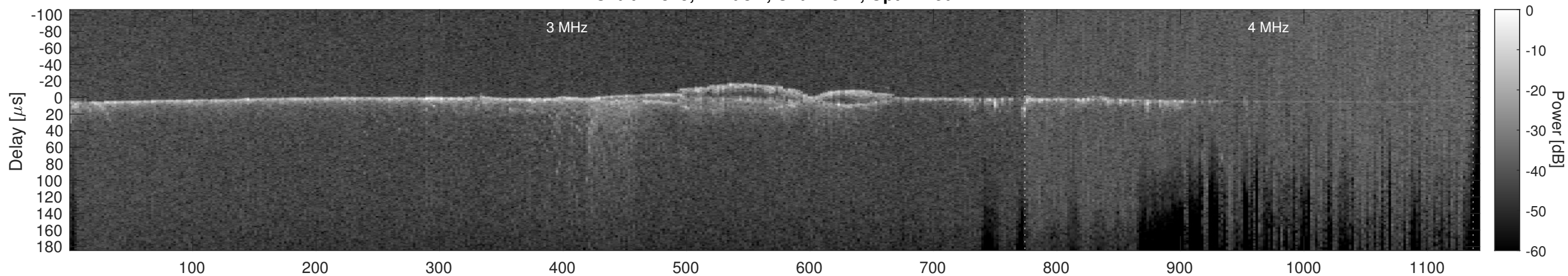
Orbit 11875, Cluttergram
