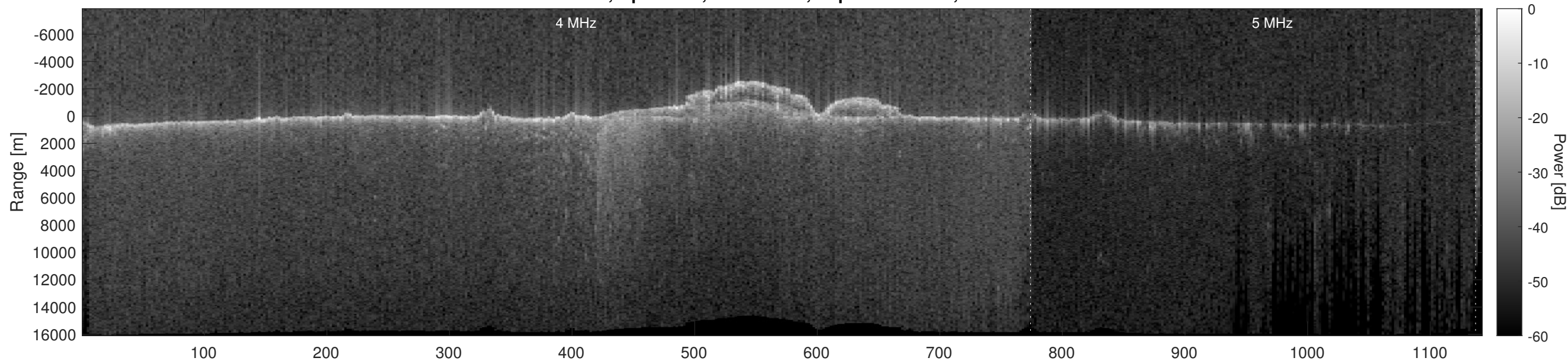
Orbit 11875, Optimized, No Window, Depth-Corrected, Channel 2
