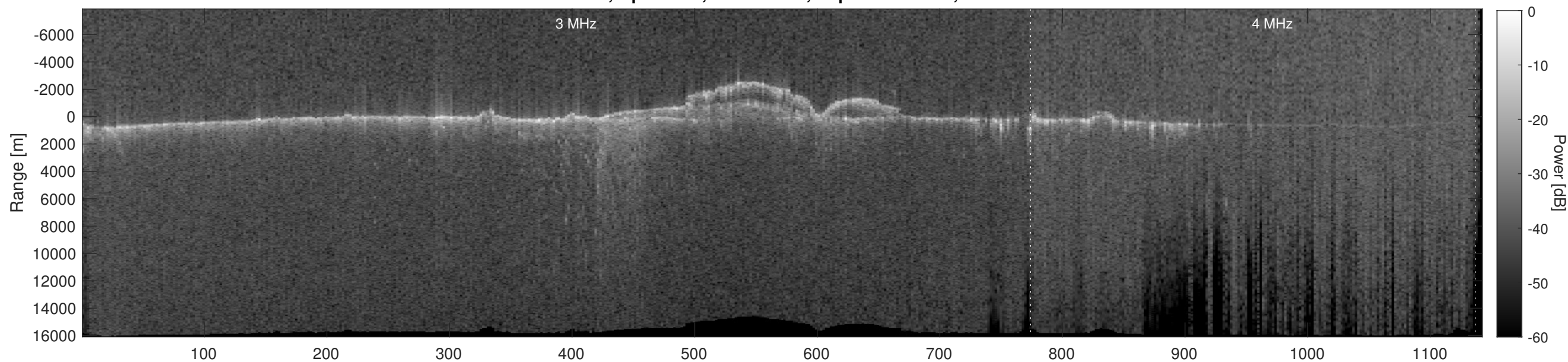
Orbit 11875, Depth-Corrected Cluttergram
