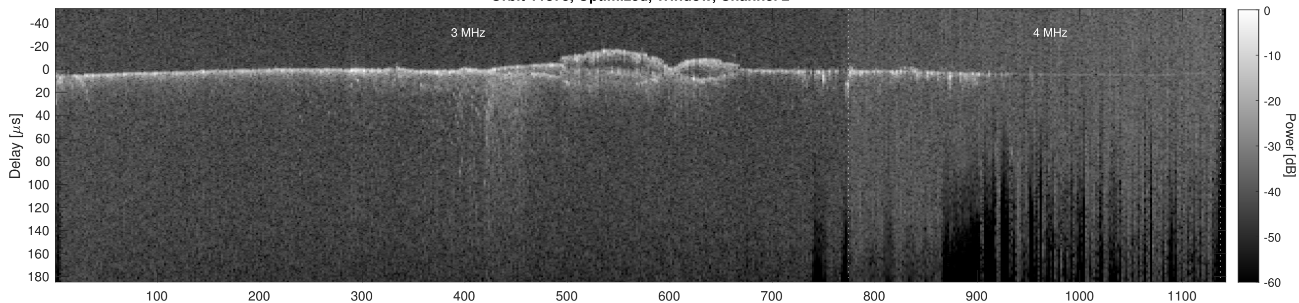
Orbit 11875, Cluttergram
