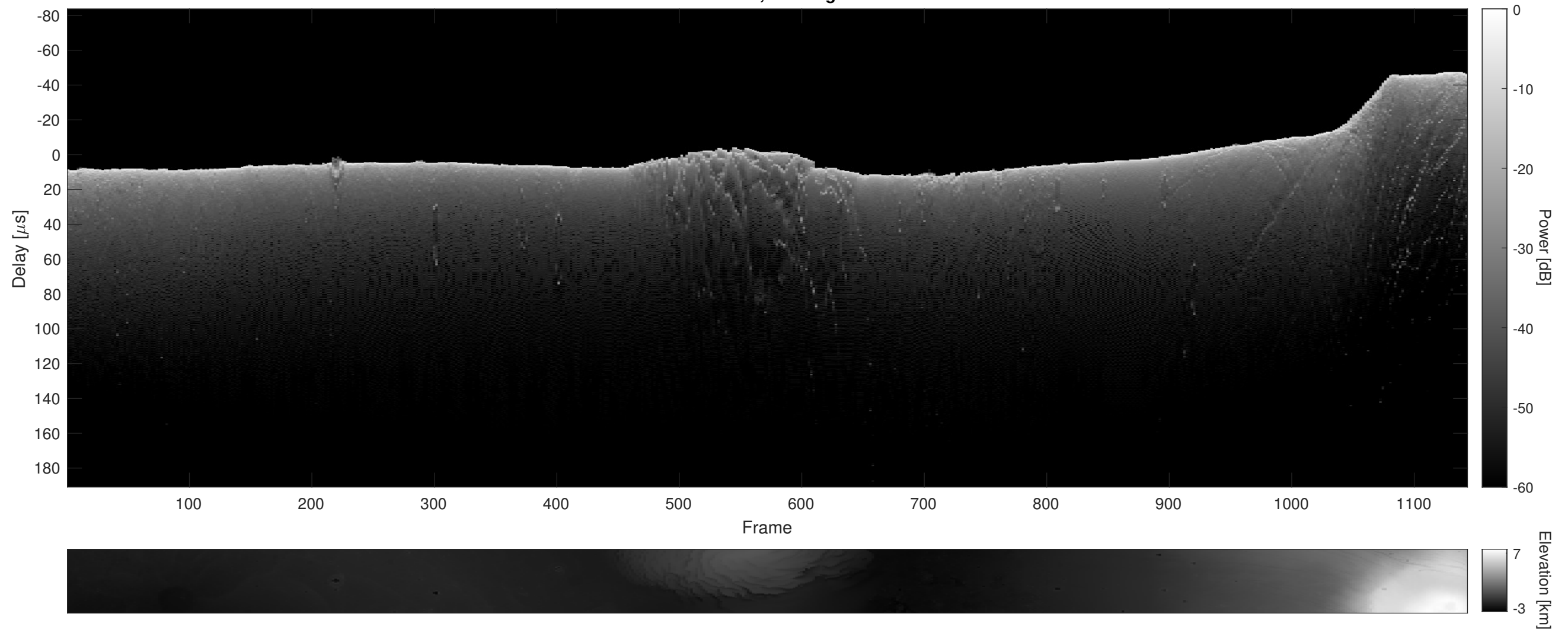
Orbit 11876, Cluttergram
