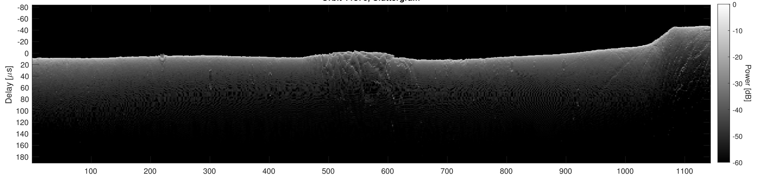
Orbit 11876, Cluttergram
