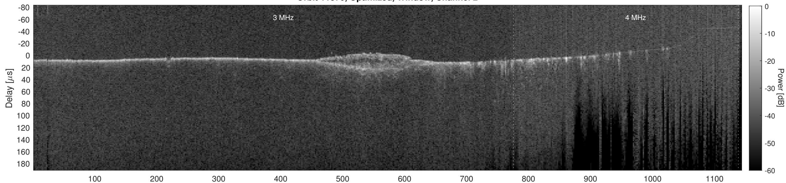
Orbit 11876, Cluttergram
