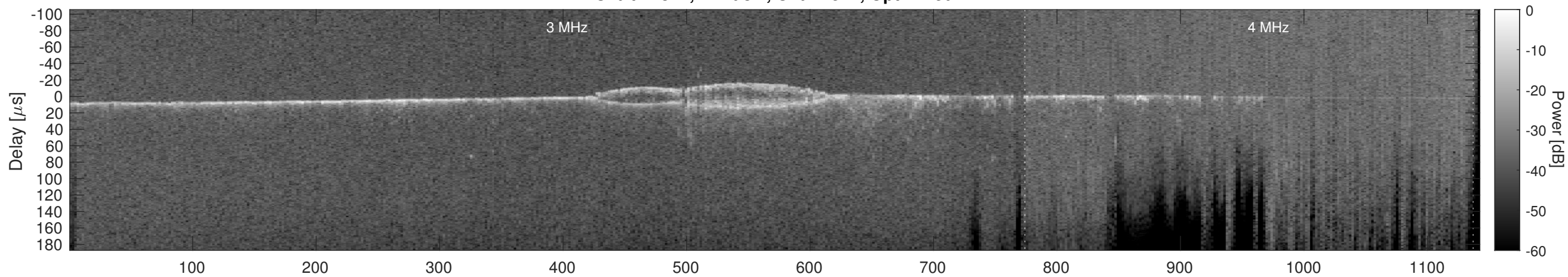
Orbit 11877, Cluttergram
