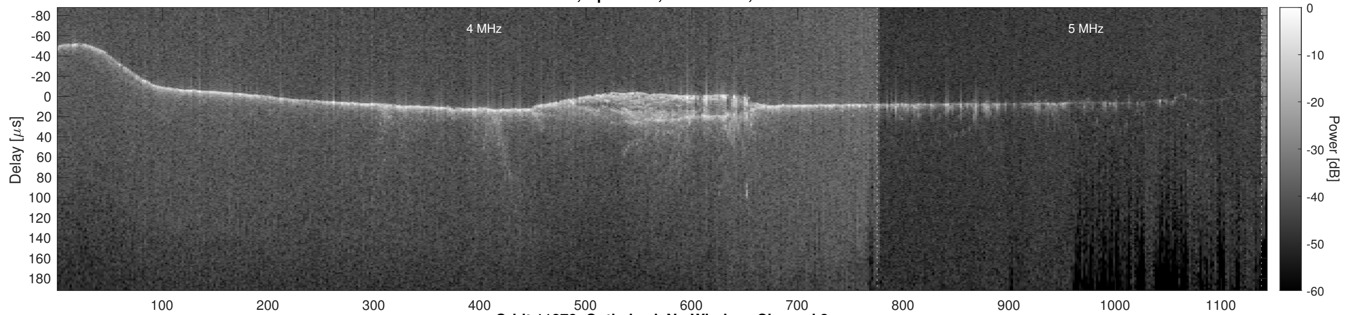
Orbit 11878, Optimized, No Window, Channel 2
