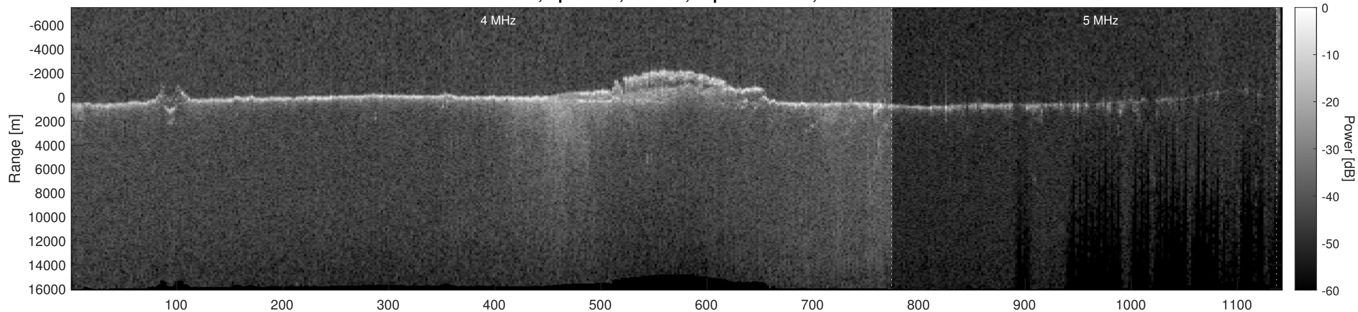
Orbit 11879, Optimized, Window, Depth-Corrected, Channel 2
