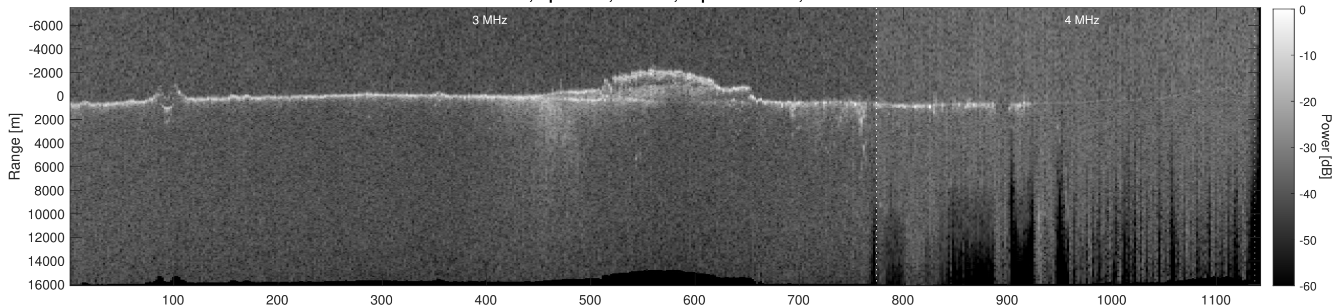
Orbit 11879, Depth-Corrected Cluttergram
