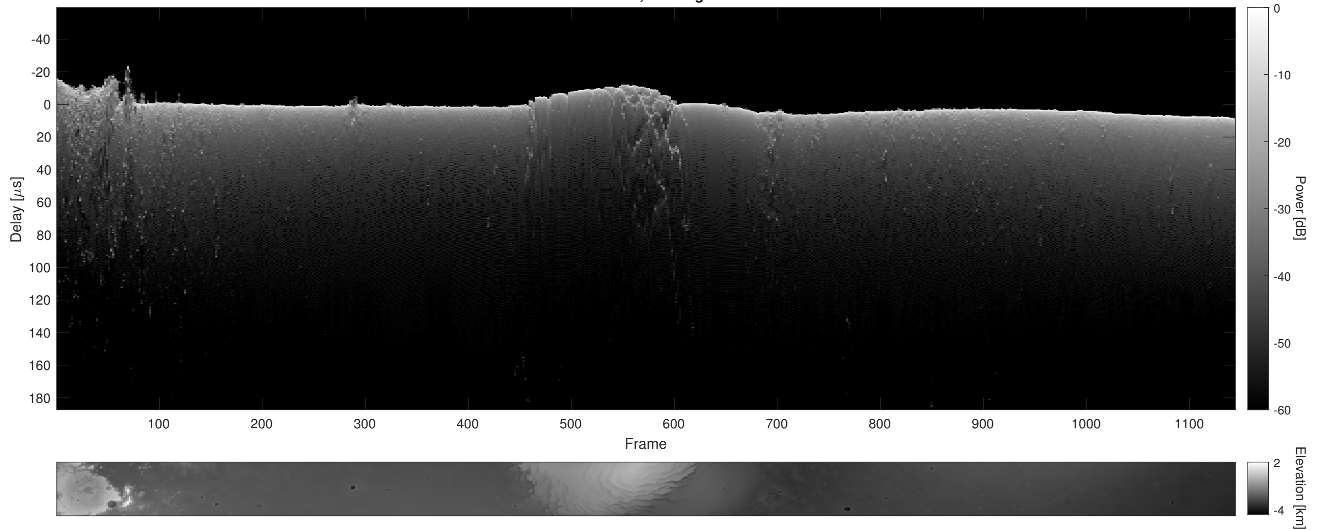
Orbit 11880, Cluttergram
