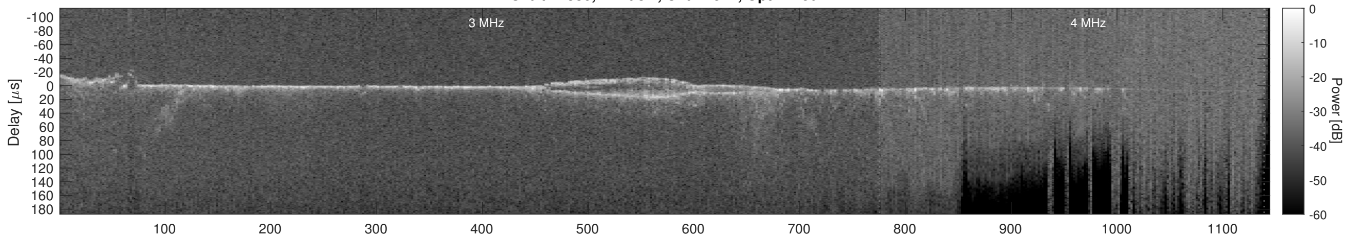
Orbit 11880, Cluttergram
