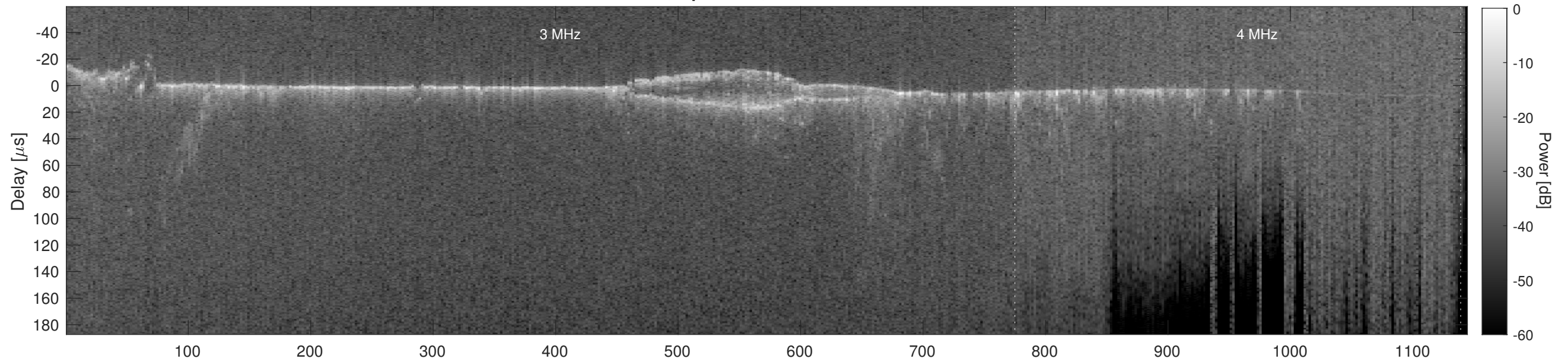
Orbit 11880, Cluttergram
