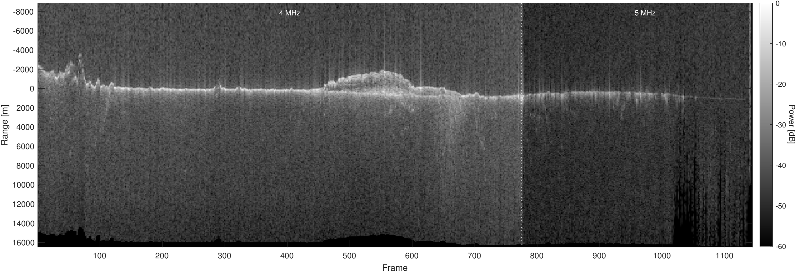
Orbit 11880, Optimized, No Window, Depth-Corrected, Channel 2
