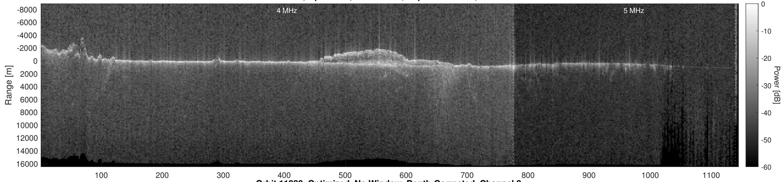
Orbit 11880, Optimized, No Window, Depth-Corrected, Channel 2
