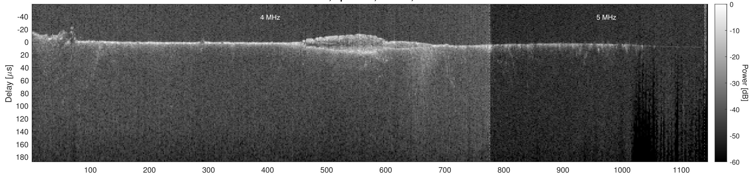
Orbit 11880, Optimized, Window, Channel 2
