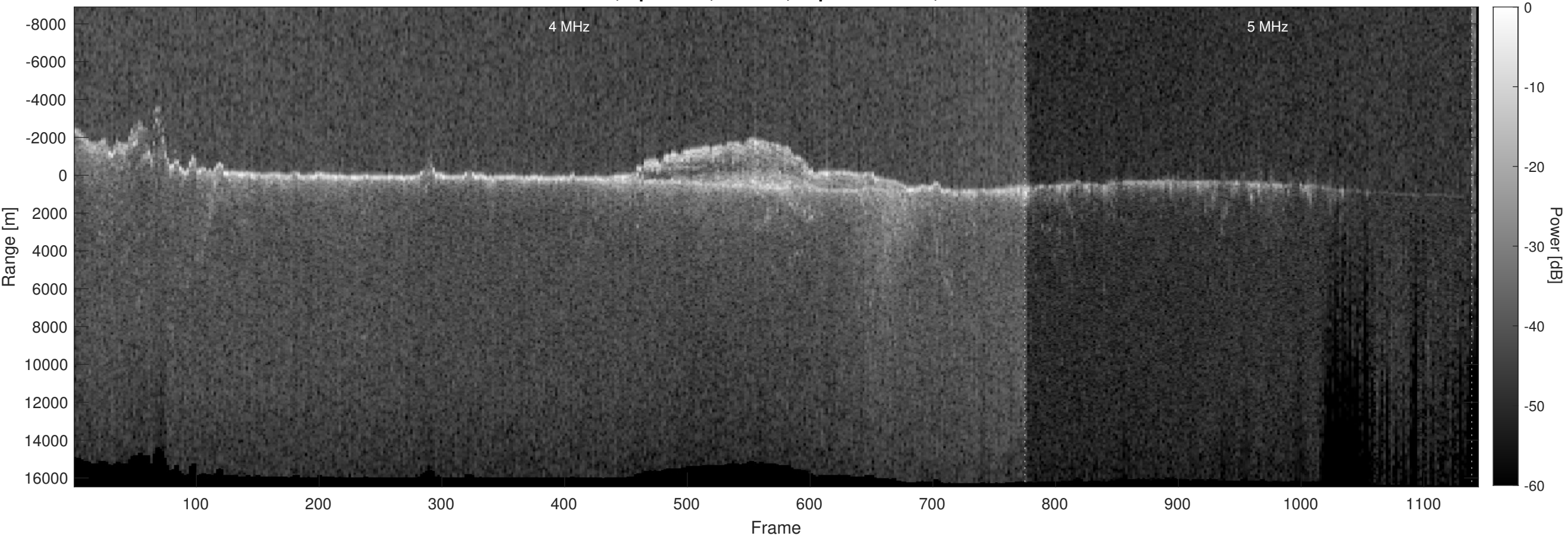
Orbit 11880, Optimized, Window, Depth-Corrected, Channel 2
