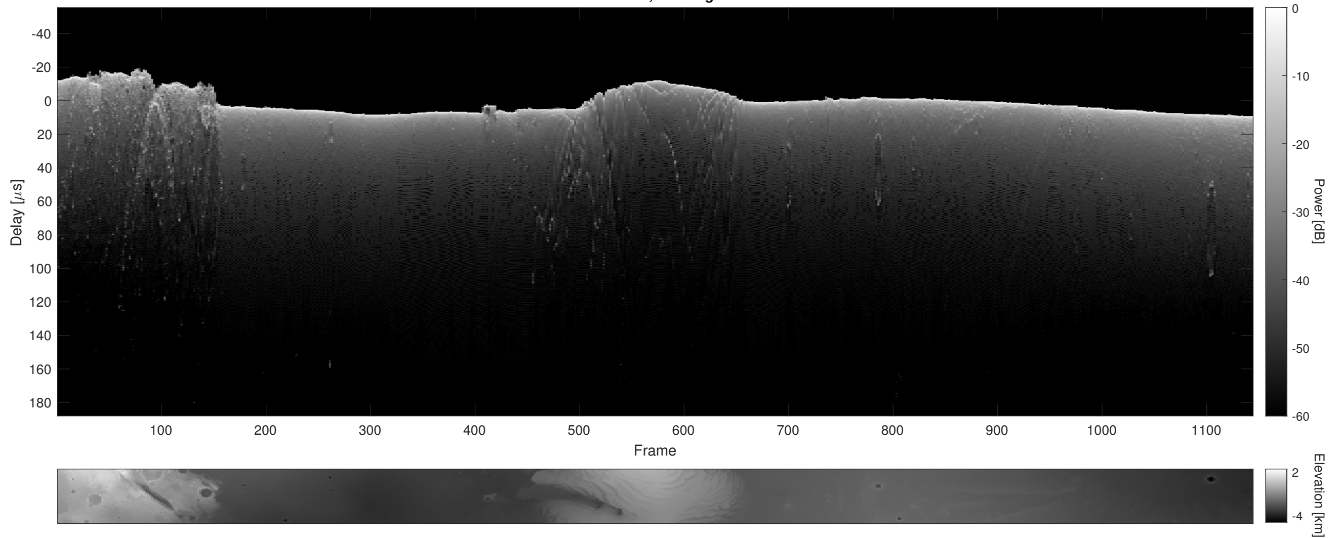
Orbit 11881, Cluttergram
