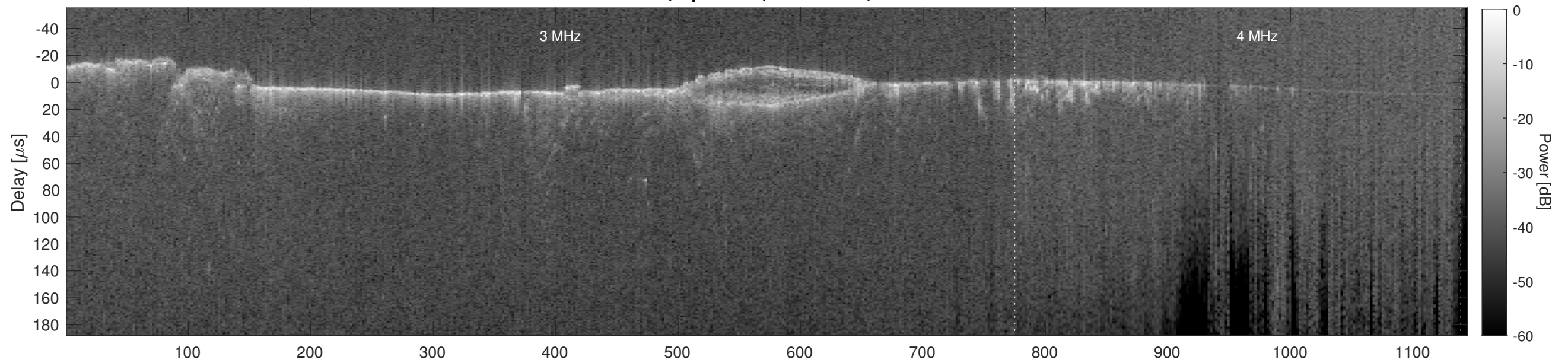
Orbit 11881, Cluttergram
