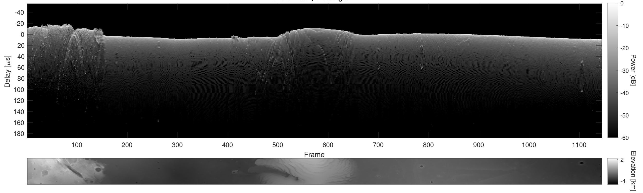
Orbit 11881, Cluttergram
