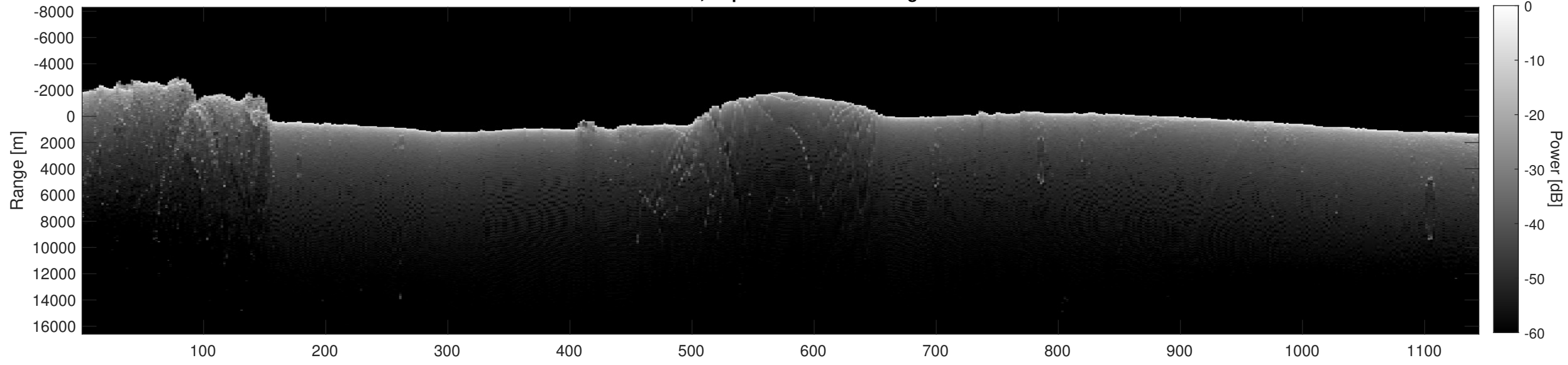
Orbit 11881, Depth-Corrected Cluttergram
