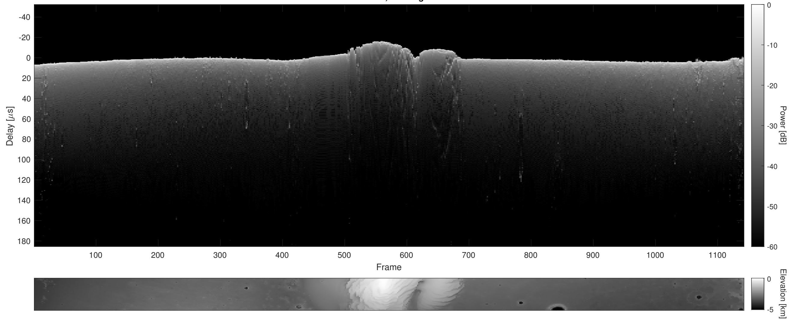
Orbit 11882, Cluttergram
