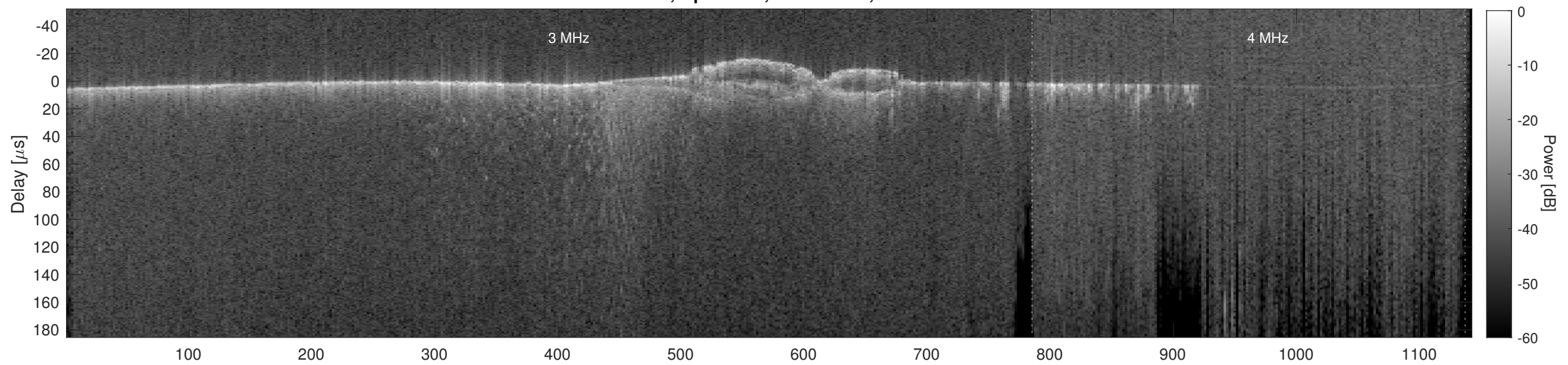
Orbit 11882, Cluttergram
