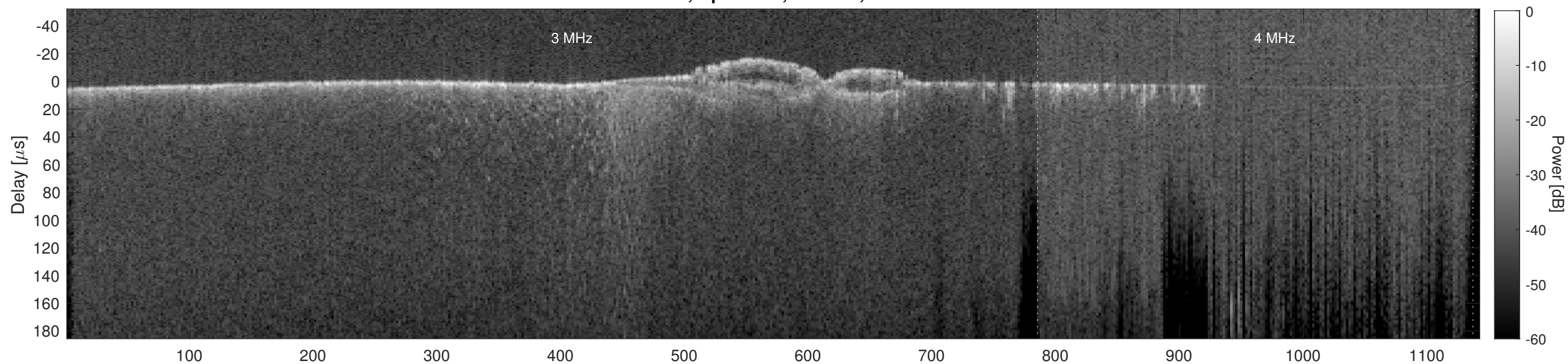
Orbit 11882, Cluttergram
