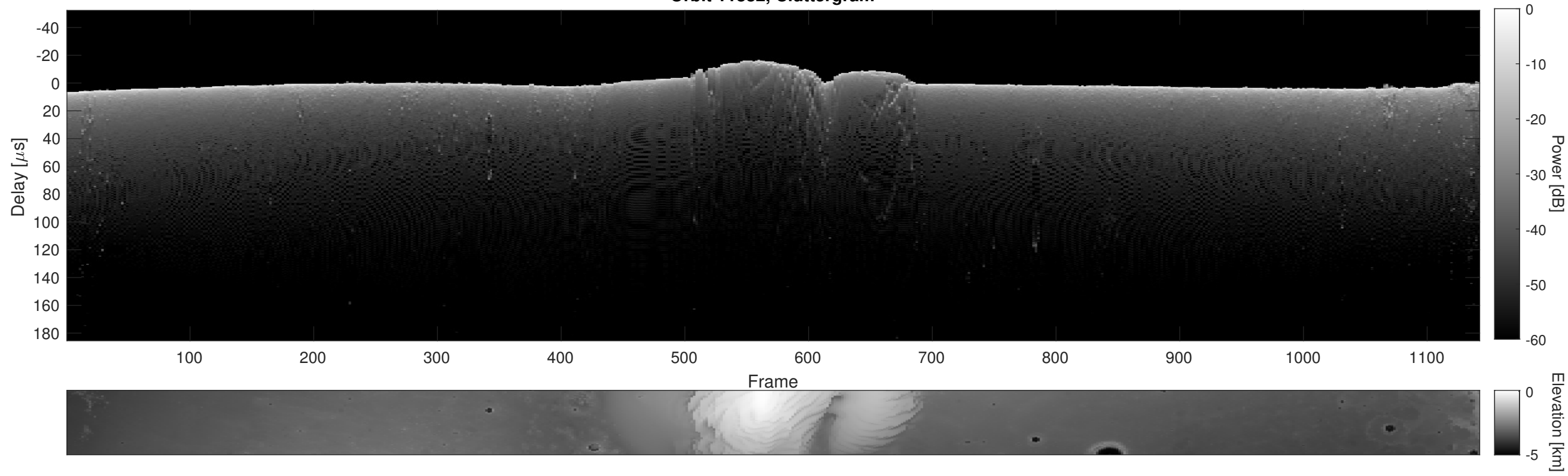
Orbit 11882, Cluttergram
