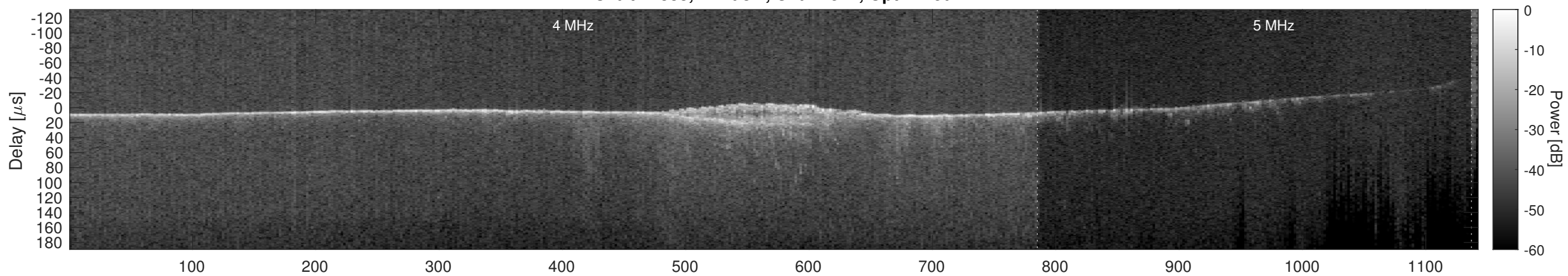
Orbit 11883, Cluttergram
