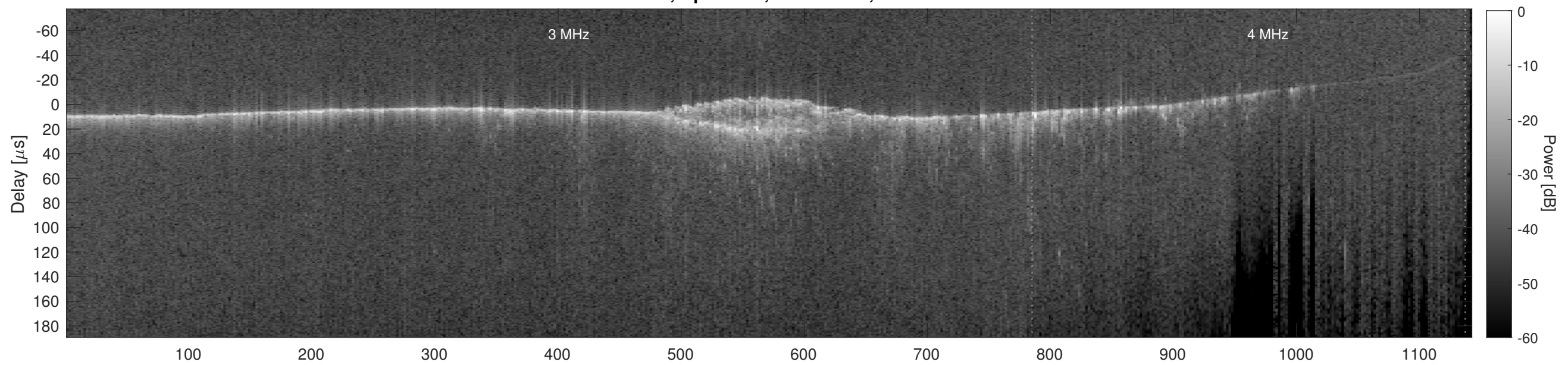
Orbit 11883, Cluttergram
