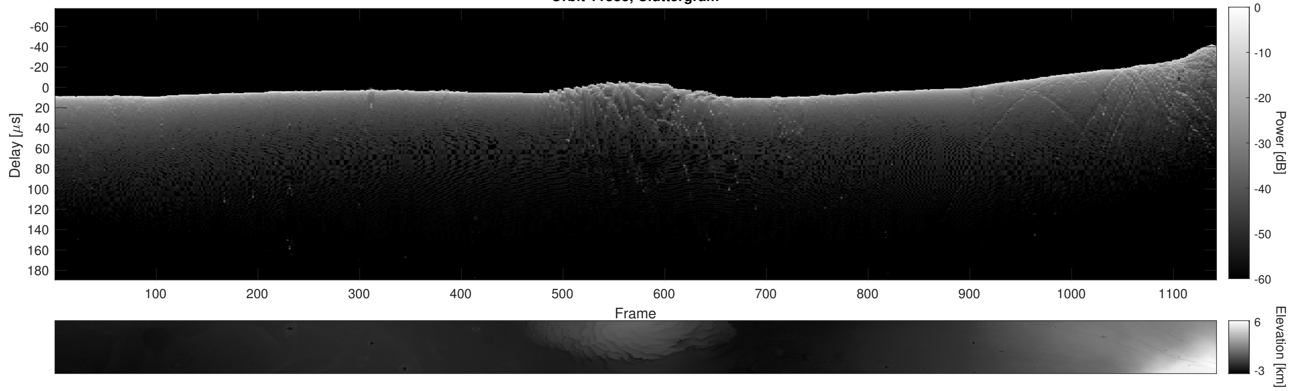
Orbit 11883, Cluttergram
