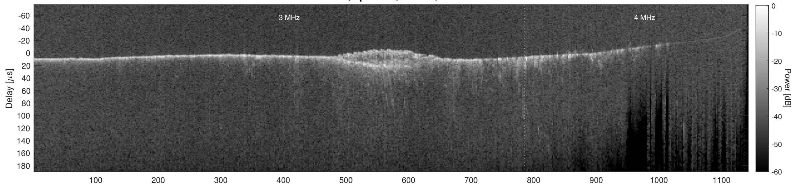
Orbit 11883, Cluttergram
