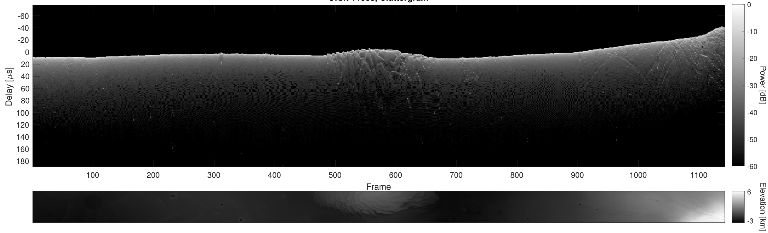
Orbit 11883, Cluttergram
